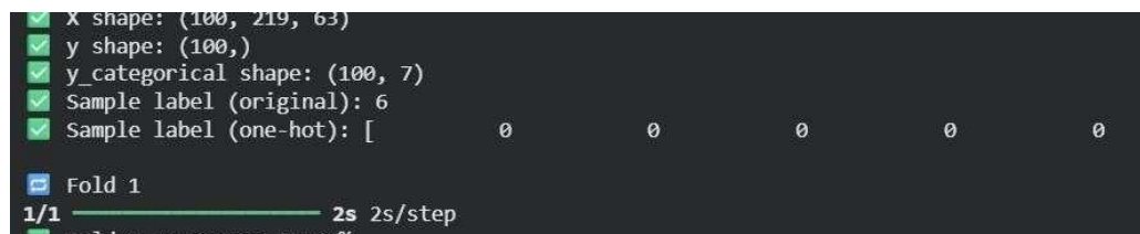
Fig. 8.4 K-fold cross validation
